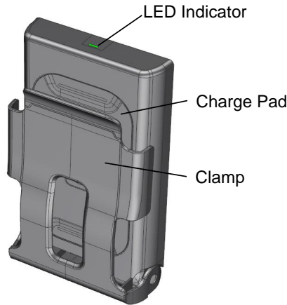
Figure 2.0: Wireless Charger
