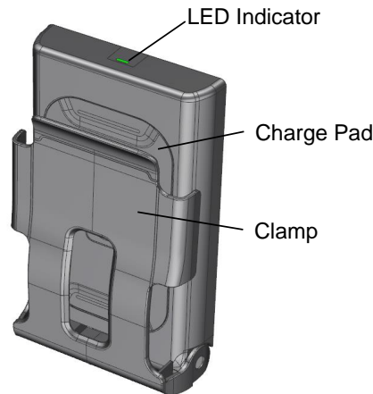
Figure 2.0: Wireless Charger
